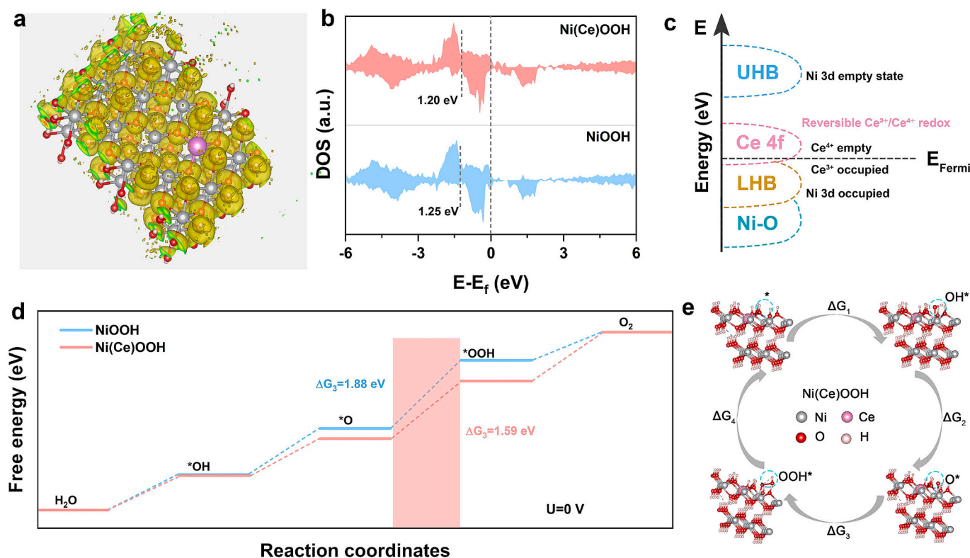
Fig. 5. (a) Spatial charge-density distribution of Ni(Ce)OOH. Colour code: Ni in argent, Ce in pink, O in red, H in white; electron-rich and electron-deficient regions are denoted by chartreuse and colorless shading, respectively. (b) Computed density-of-states (DOS) profiles for the Ni 3d orbital in Ni(Ce)OOH and pristine NiOOH. (c) Energy-level schematic for Ce-doped NiOOH. (d) OER Gibbs free-energy profiles comparing Ni(Ce)OOH with NiOOH. (e) Reaction-pathway schematic illustrating the OER catalytic mechanism on Ni(Ce)OOH. (For interpretation of the references to colour in this figure legend, the reader is referred to the web version of this article.)
